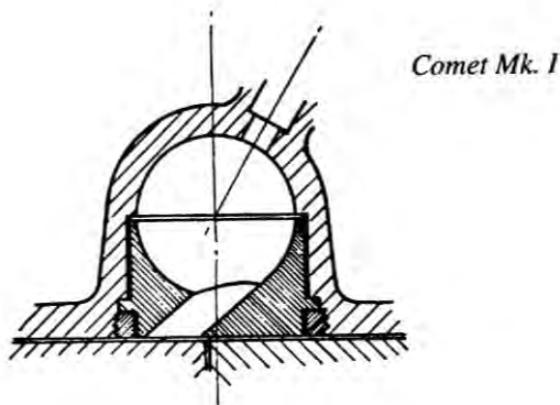
Figure 11. Cross section of first Comet IDI diesel combustion chamber.
